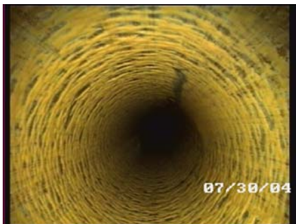
Figure 9 Stainless Steel Condenser Tube with Calcium Carbonate Scale
