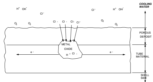
Figure 1 Model of Under-deposit Corrosion
